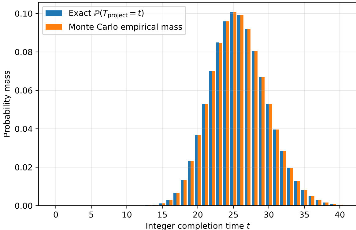
Exact discrete PMF versus Monte Carlo empirical PMF
